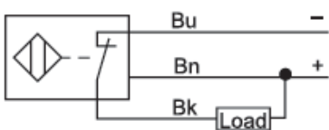
NPN NC
