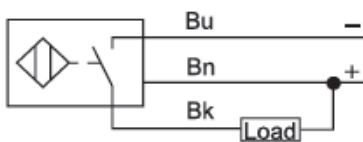
NPN NO
