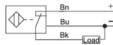
PNP NC
